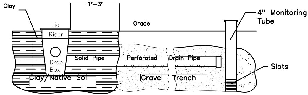
Trench Detail (pg 2 of 2)
